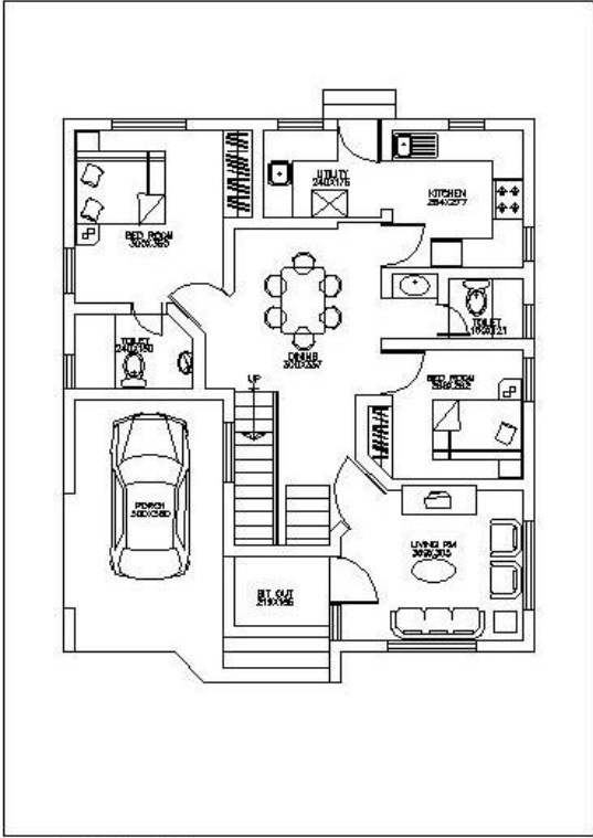
GROUND FLOOR PLAN G F :- 1068 Sqft F F :- 608 Sqft TOTAL :- 1676 Sqft 17 x 12 south facing
